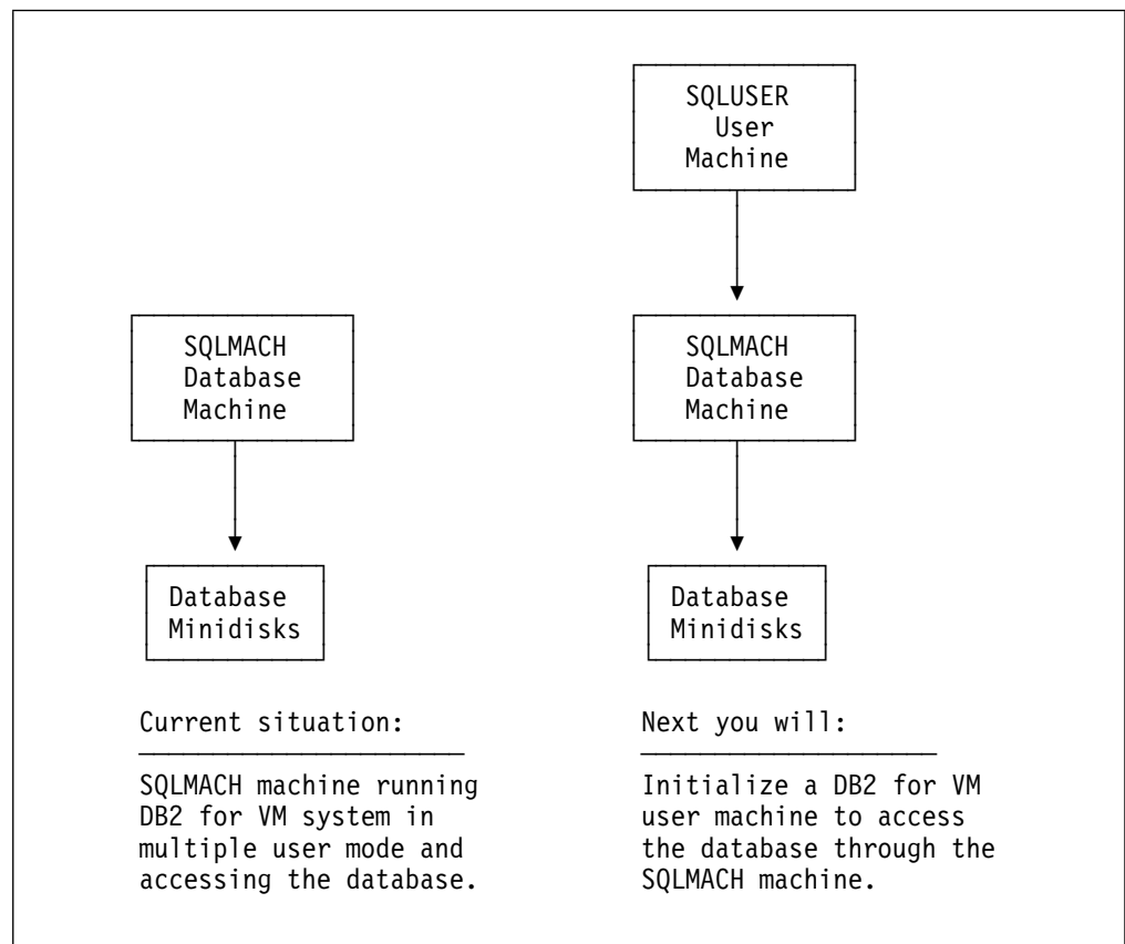
Figure 18. Installation Environment
