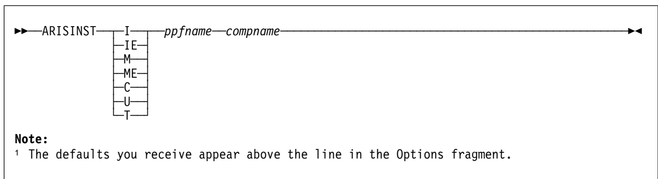
Figure 24. ARISINST syntax
