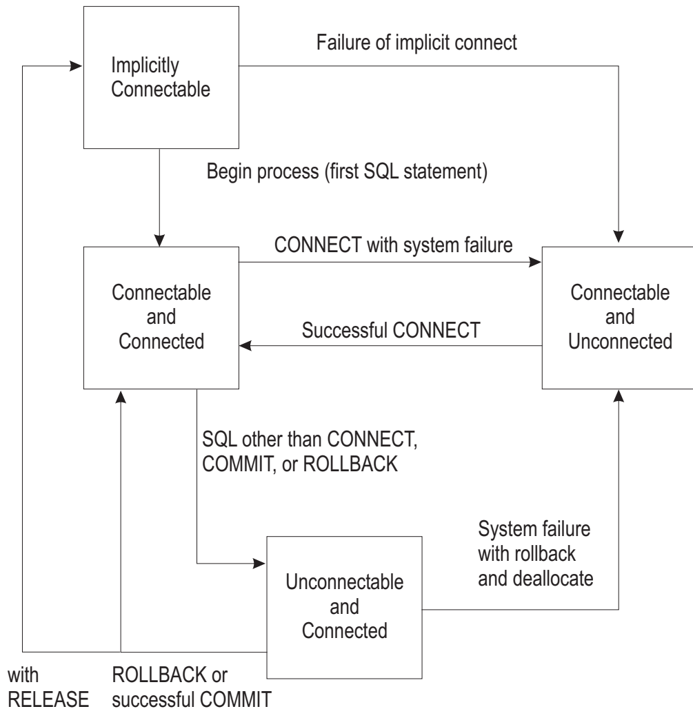
Figure 7. VM Connection State Transitions
