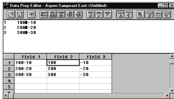
Figure 22-6: New 100-10 Field
