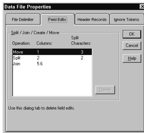
Figure 20-7: Field Operations
