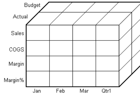
Figure 24-5: Three-Dimensional Database
