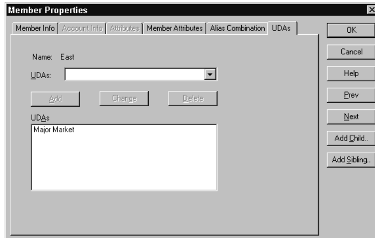
Figure 8-13: UDAs Page
