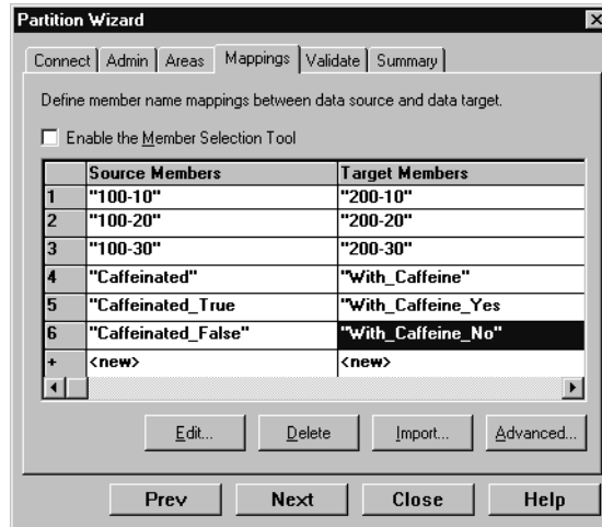
Figure 14-19: Mapping Attributes
