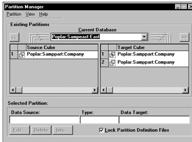
Figure 14-1: Partition Manager
