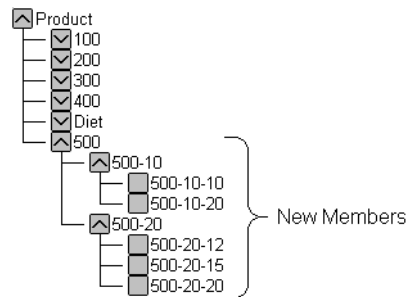
Figure 18-3: Generation References
