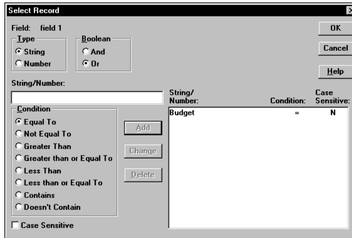
Figure 20-8: Selecting Records
