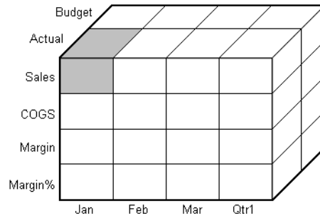
Figure 2-9: Sales -> Jan -> Actual Slice of the Database
