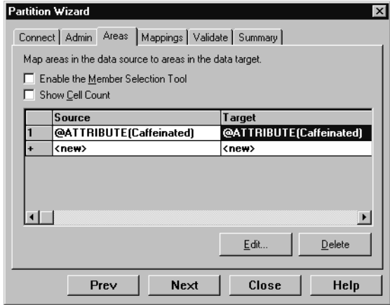
Figure 13-12: Correct Partitioning
