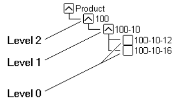
Figure 2-4: Levels
