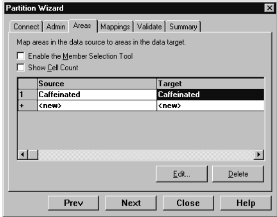
Figure 13-11: Incorrect Partitioning
