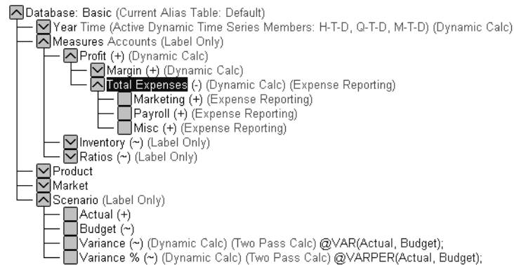
Figure 25-24: Sample Basic Showing Expense Items
