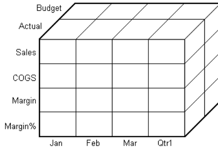
Figure 2-6: Three-Dimensional Database
