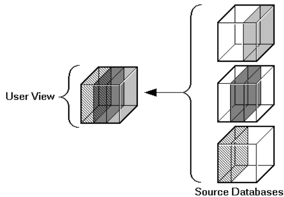
Figure 13-6: Transparent Partitions
