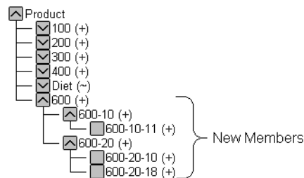
Figure 18-7: Levels
