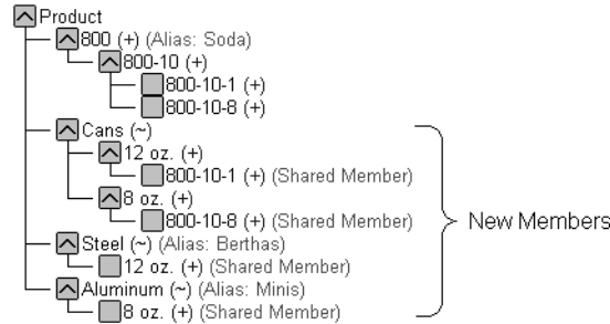
Figure 18-42: Multiple Roll-Ups
