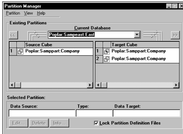
Figure 14-32: Partition Manager
