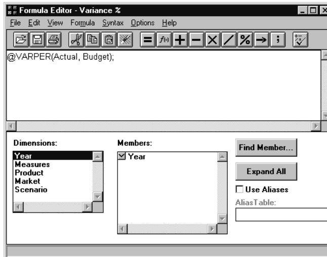
Figure 8-16: Formula Editor
