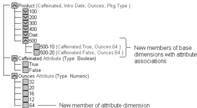
Figure 18-18: Associating Attributes
