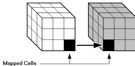
Figure 13-9: Linked Partition
