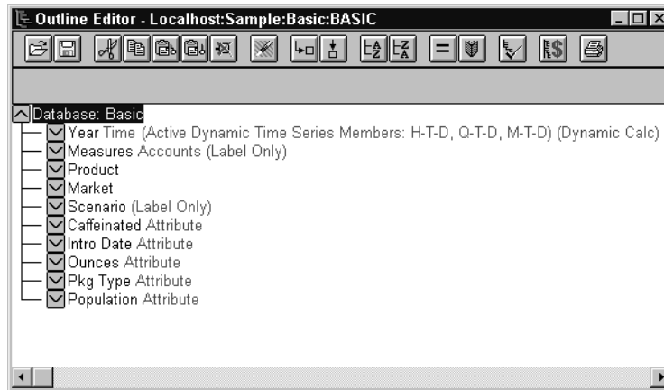
Figure 7-2: Outline Editor
