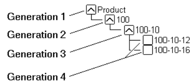
Figure 2-3: Generations
