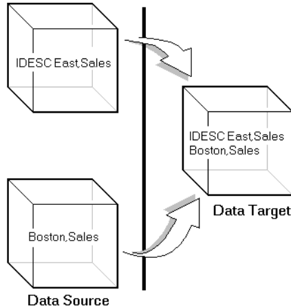
Figure 13-3: Overlapping Partitions
