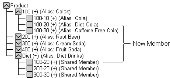
Figure 18-26: Shared Members in the Sample Basic Database
