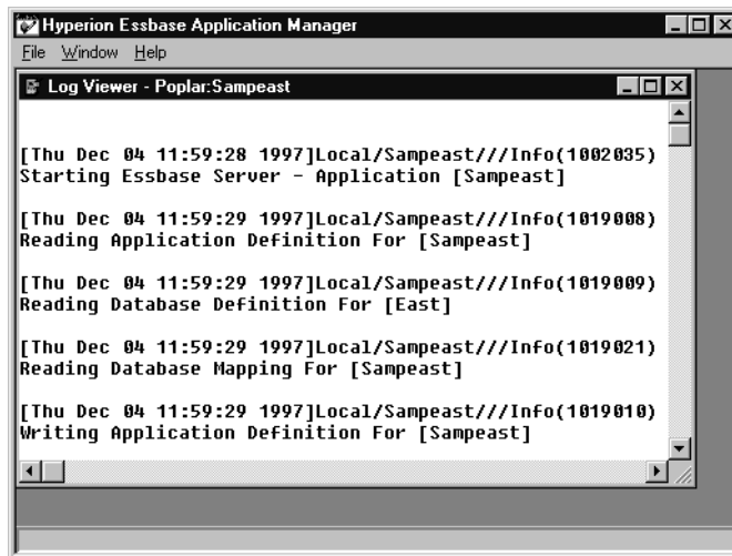
Figure 41-8: Sample Application Log
