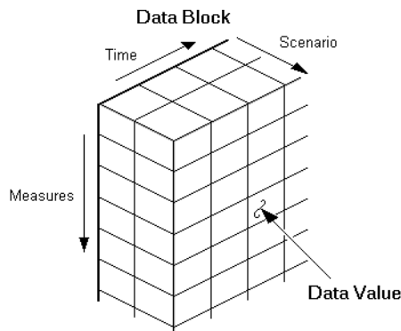
Figure 3-4: Part of a Data Block for the Sample Basic Database
