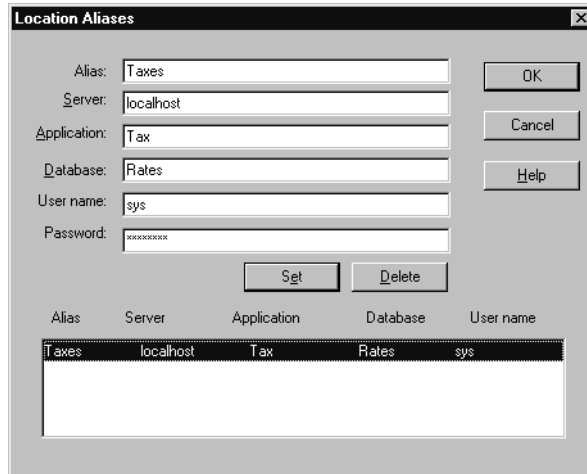
Figure 6-13: Creating a Location Alias
