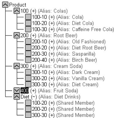
Figure 27-12: Calculating Shared Members
