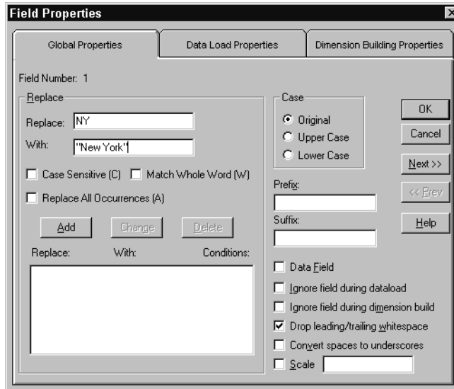
Figure 22-11: Global Properties Page: Replace Box
