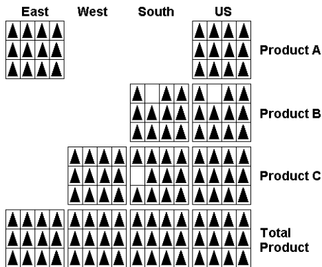
Figure 3-12: Data Blocks Created for Sparse Members on Region and Product
