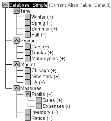
Figure 2-15: Adding Stored Members to the Outline
