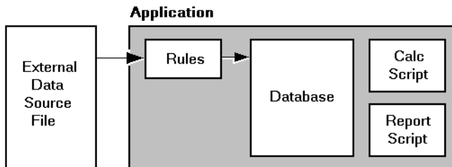
Figure 6-1: Parts of an Essbase Application
