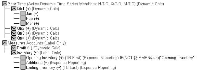
Figure 29-3: Sample Basic Outline Showing First Tag
