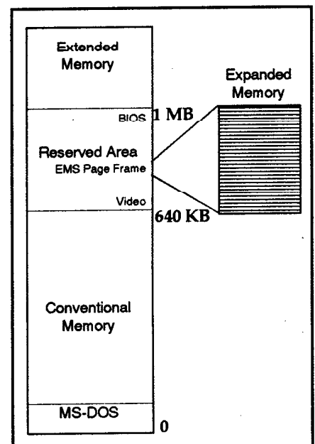
Figure 1. The MS-DOS computers use a unique memory scheme.
