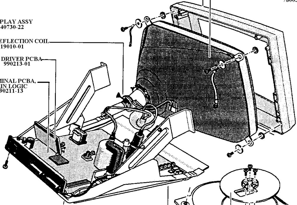
BOTTOM HOUSING ASSY 830128-03
