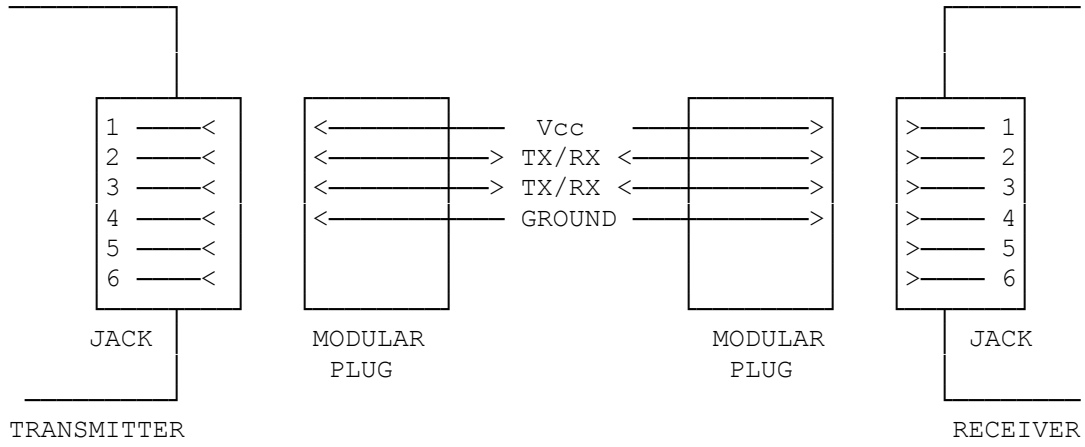
4-Wire Application: RJ-11 Modular Connector
